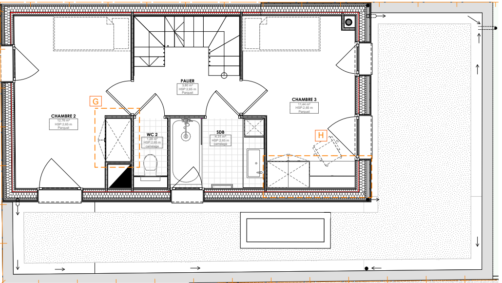
Plan R+1
